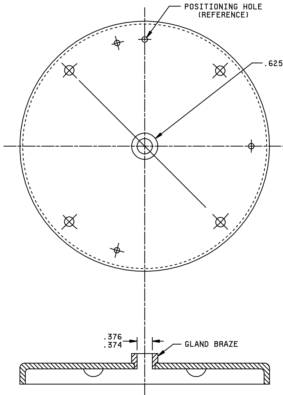
FIGURE 3. Cover assembly.
