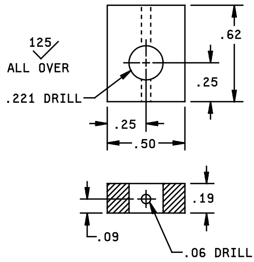
FIGURE 8. Coupler plate. (09)
