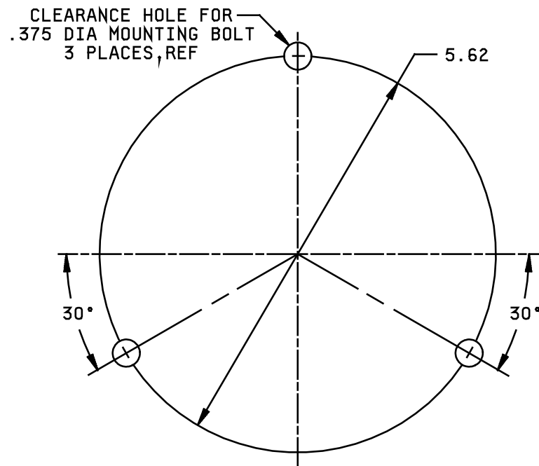
FIGURE 9. Mounting dimensions, ref.
