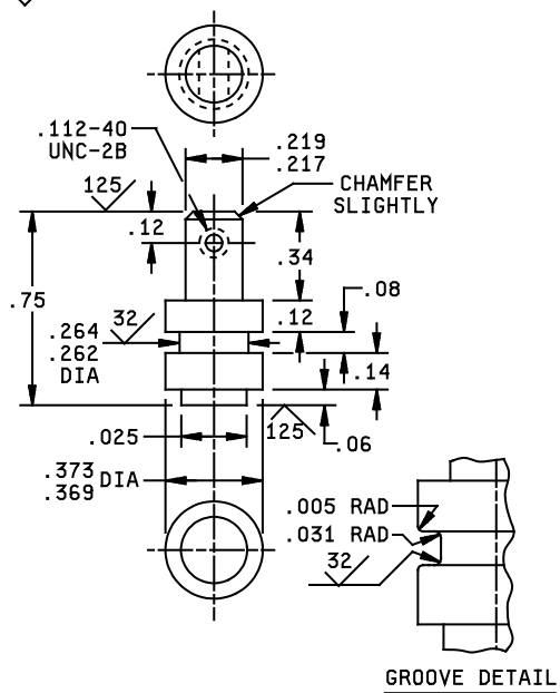
FIGURE 6. Shaft. (07)
