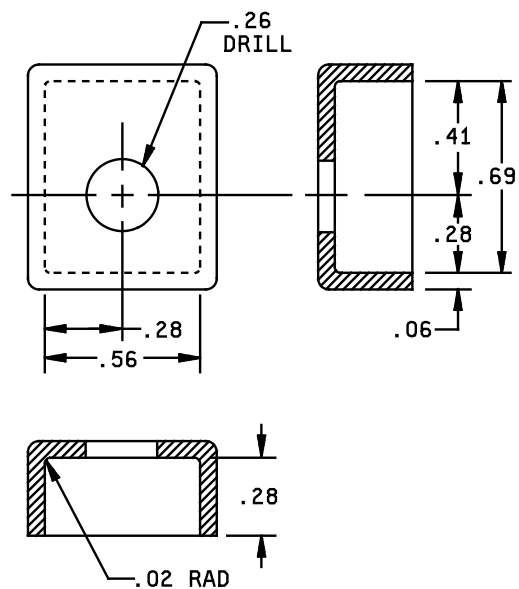
FIGURE 7. Coupler. (08)
