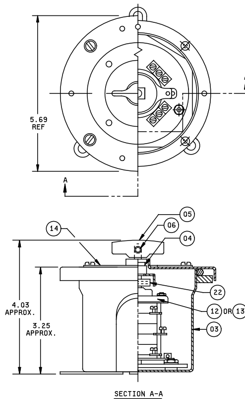
FIGURE 1. Switch, enclosed. (01, 02 (-002 shown))
