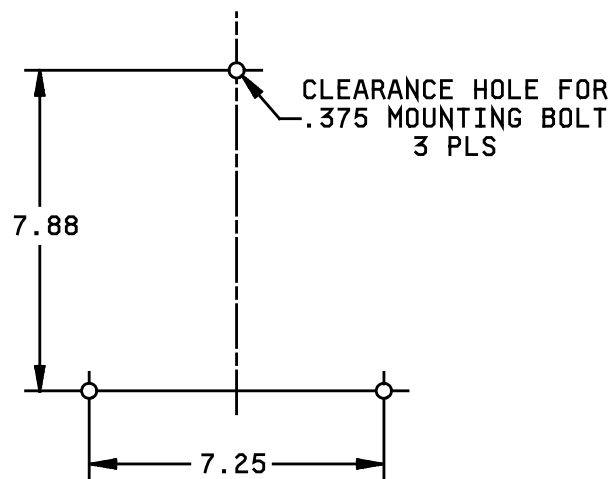
FIGURE 9. Mounting dimensions, ref.
