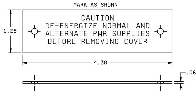
FIGURE 11. Caution plate. (16)
