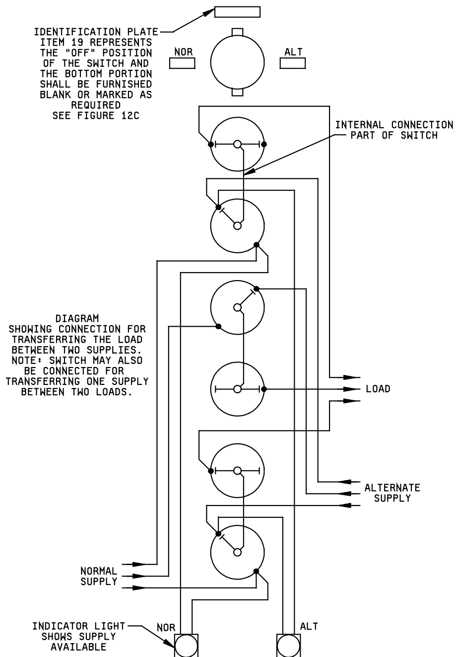
FIGURE 10. Wiring diagram. ⑨
