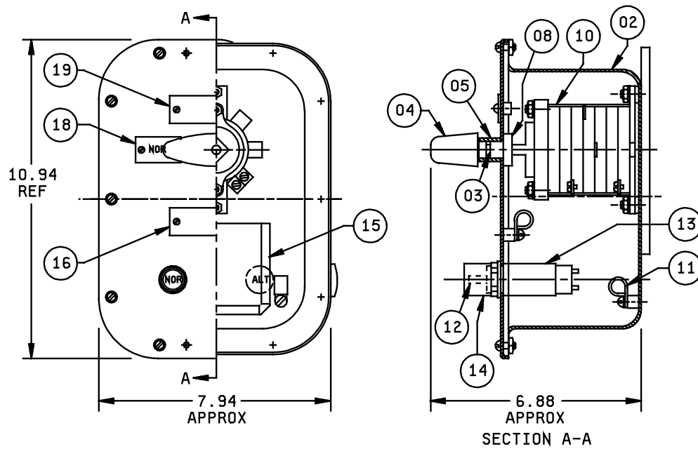
FIGURE 1. Switch, enclosed. ①
