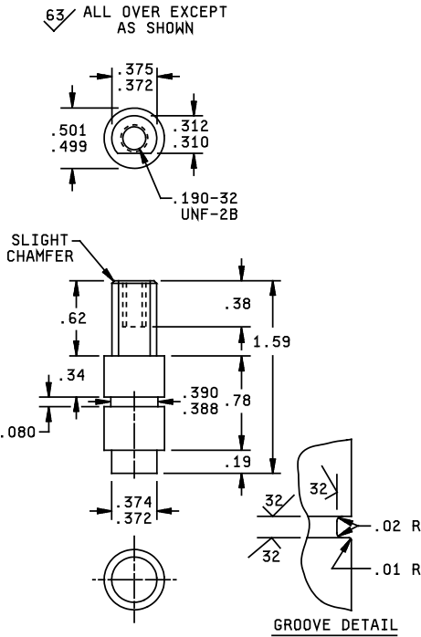
FIGURE 6. Shaft. 06
