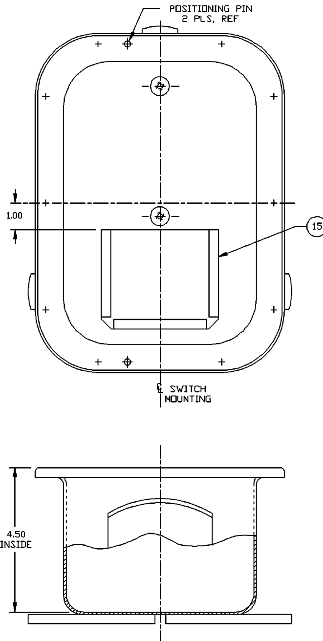
FIGURE 2. Box assembly (modified).
