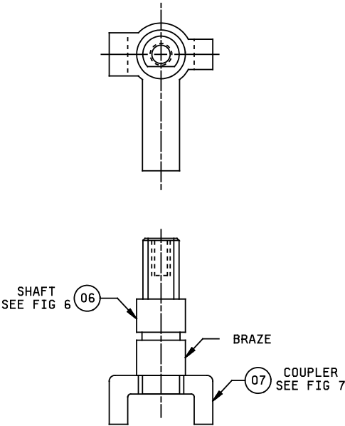
FIGURE 5. Shaft assembly. 05
