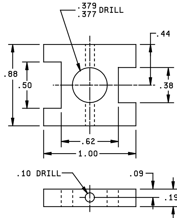
FIGURE 8. Coupler plate. (08)
