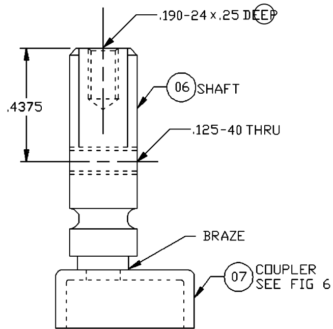
FIGURE 5. Shaft assembly. 05
