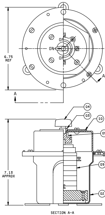
FIGURE 1. Switch, enclosed 01
