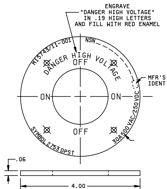
FIGURE 9. Identification plate. 10
