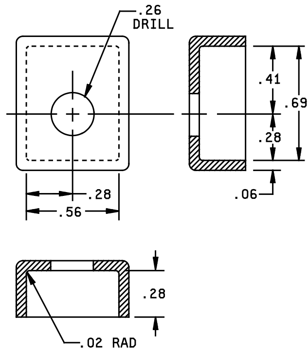
FIGURE 6. Coupler. 07
