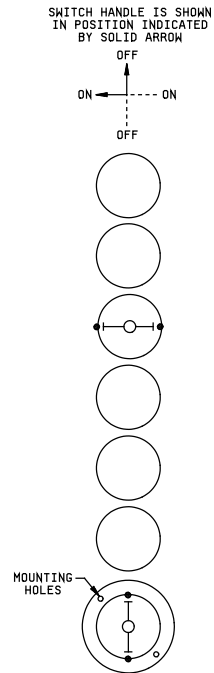
FIGURE 8. Wiring diagram. 08
