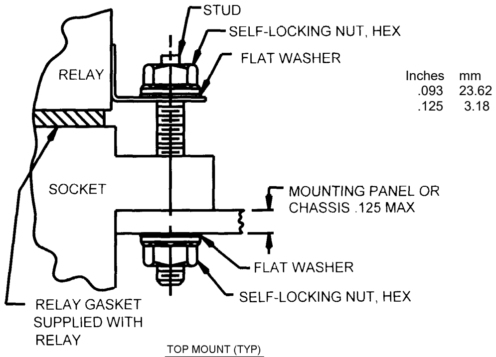
FIGURE 2. Socket mounting – Continued.
