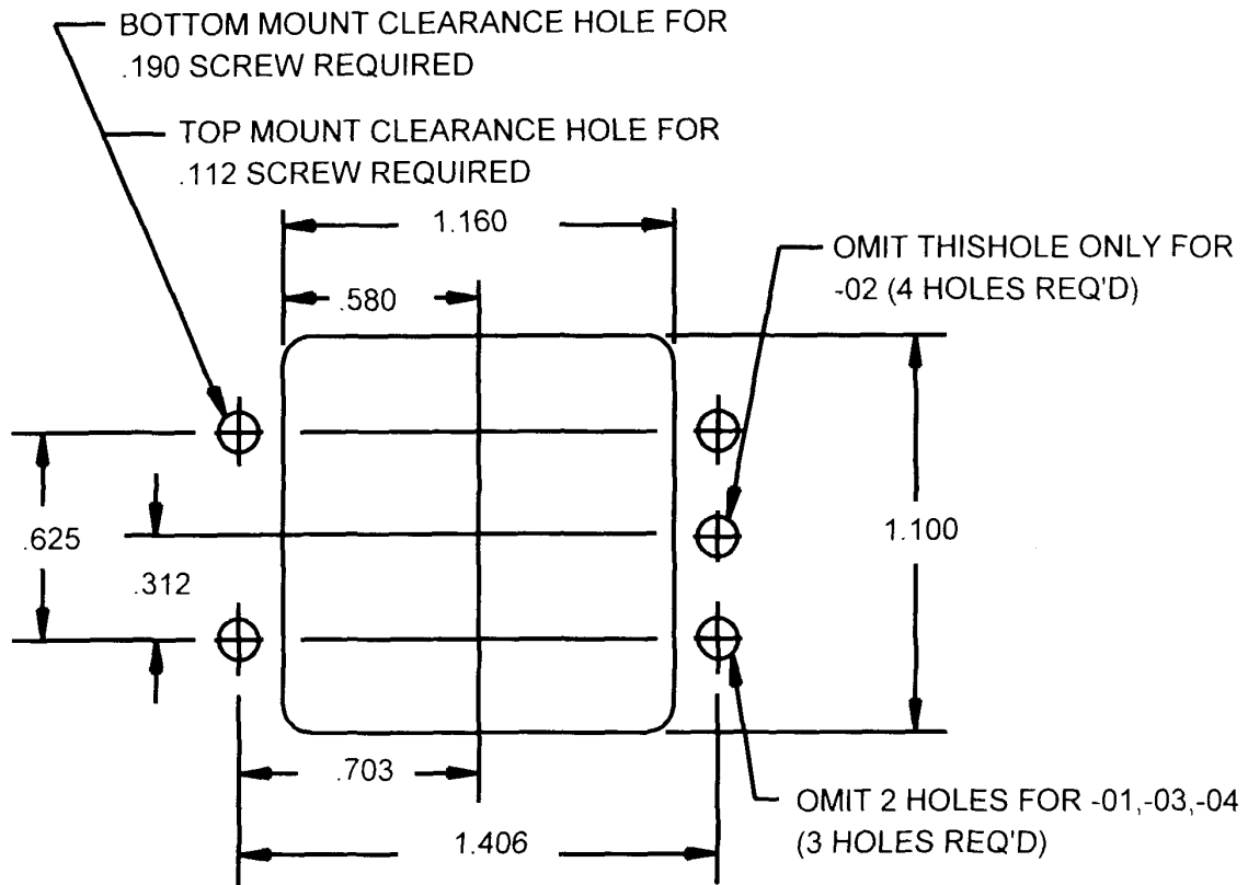
RECOMMENDED MOUNTING DIMENSIONS
