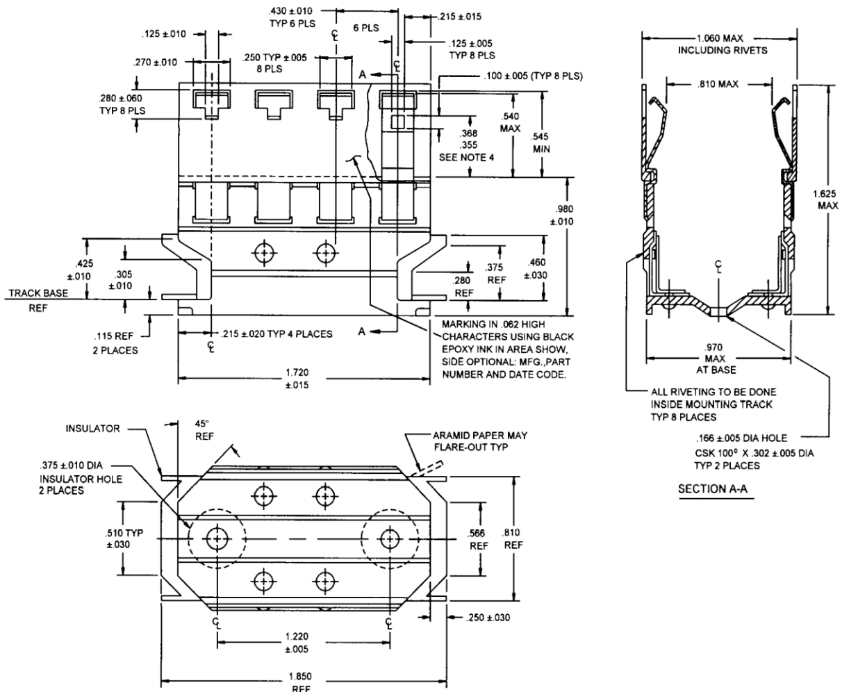
FIGURE 1. Mounting tracks.
