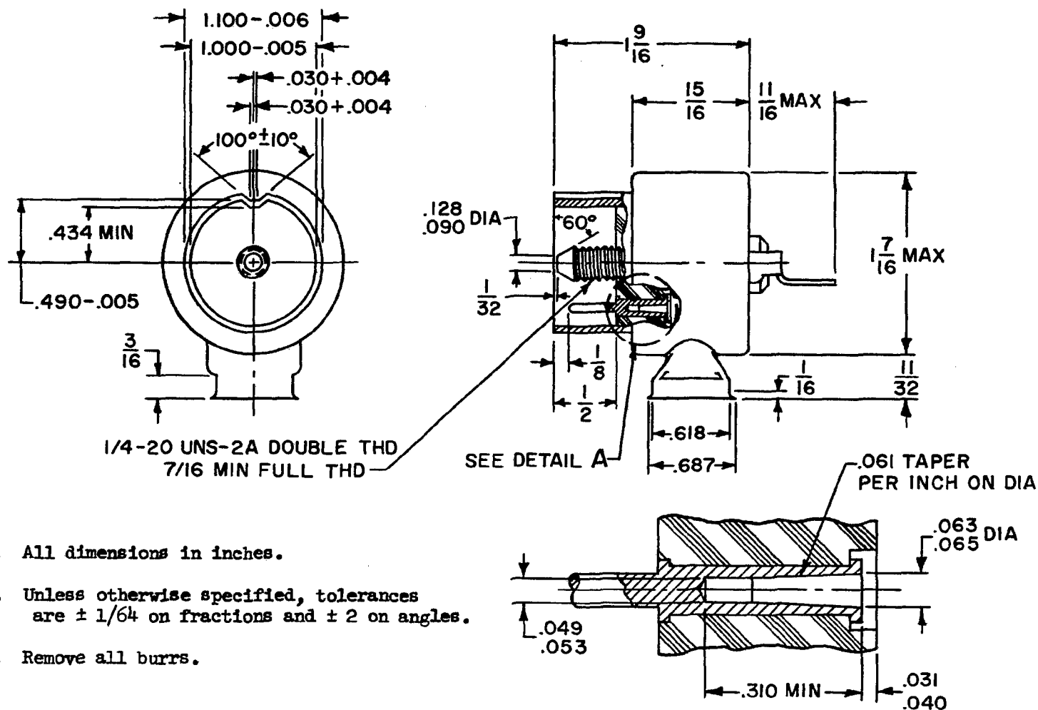
Figure 1. Plug shell and male insert dimensions.
