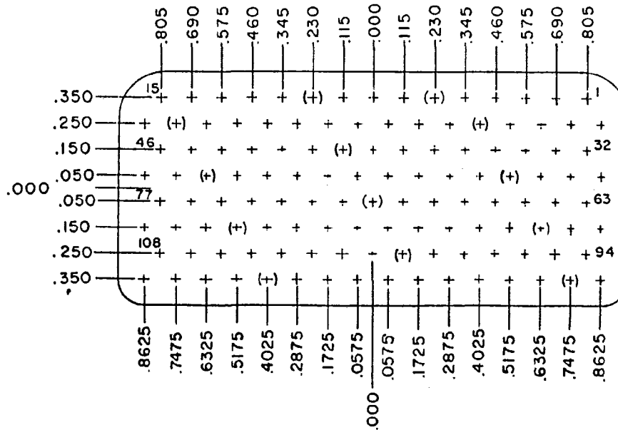
124 POSITION INSERT ARRANGEMENT 124 SIZE 20 CONTACTS SHELL DESIGNATOR B - SERVICE RATING A
