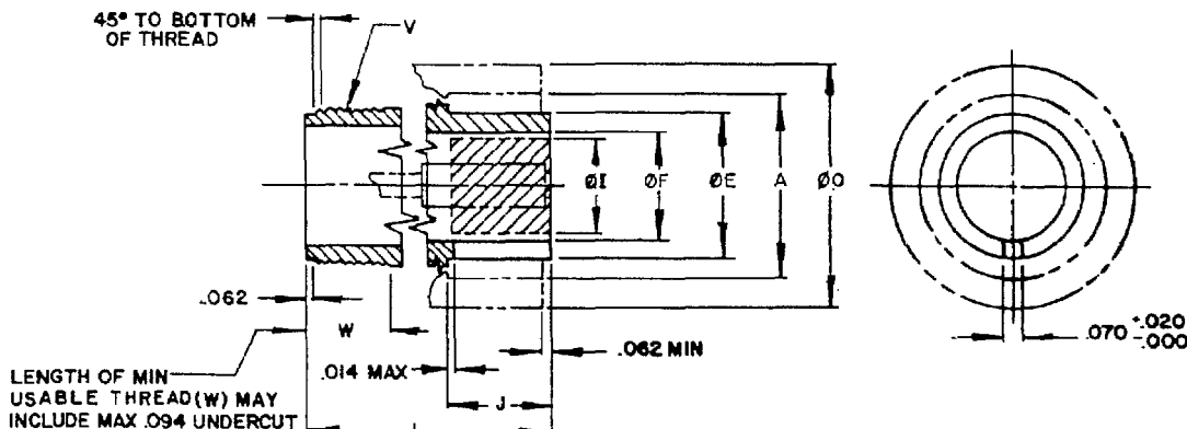
STYLE S (SOCKET INSERT) (C)
